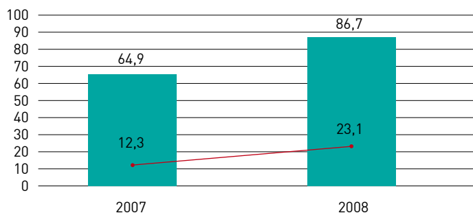
ΟΤΣ και Spark Spread (€/MWh)
